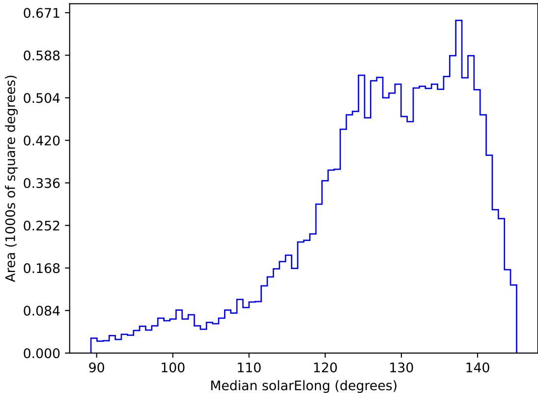
ddf_acor_sf10_lsf40_lsr20_v3.4_10yrs WFD z band: Median solarElong
