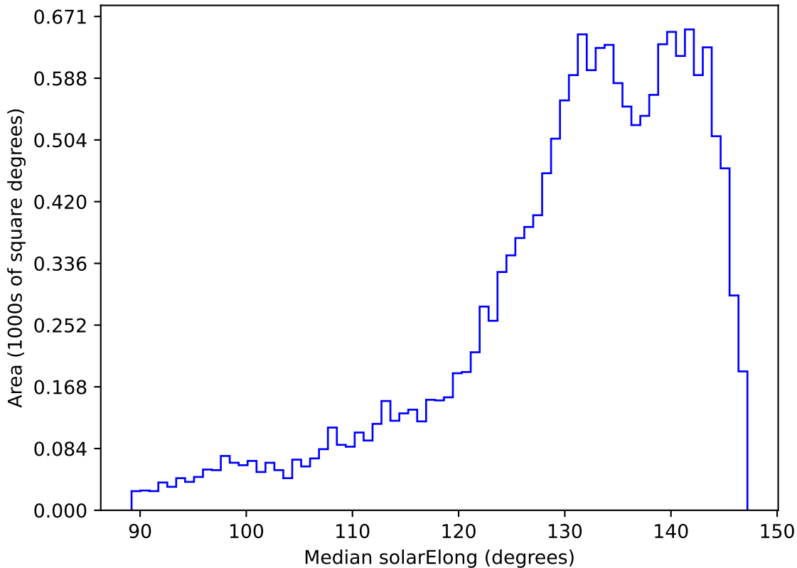
ddf_acor_sf10_lsf40_lsr20_v3.4_10yrs WFD r band: Median solarElong
