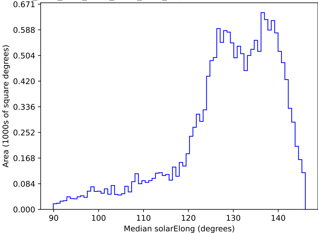
ddf_acor_sf10_lsf40_lsr20_v3.4_10yrs WFD i band: Median solarElong
