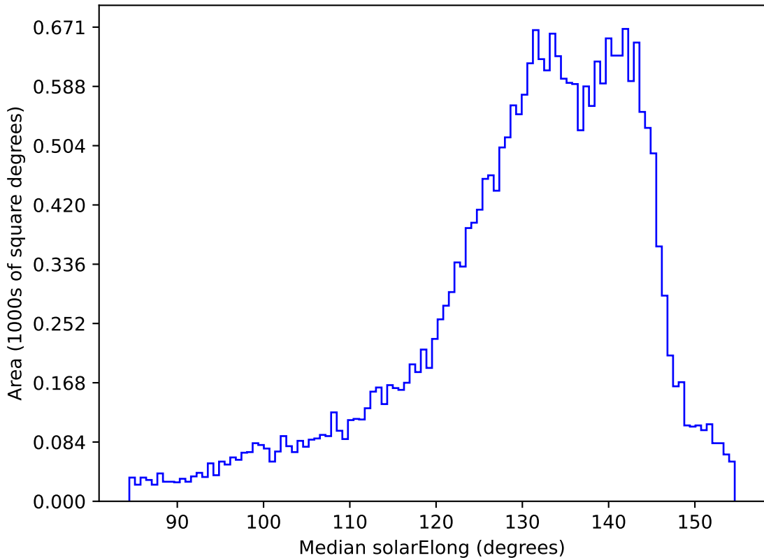
ddf_acor_sf10_lsf40_lsr20_v3.4_10yrs All sky r band: Median solarElong
