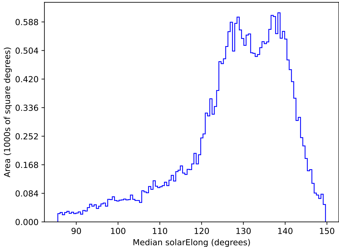
ddf_acor_sf10_lsf40_lsr20_v3.4_10yrs All sky i band: Median solarElong
