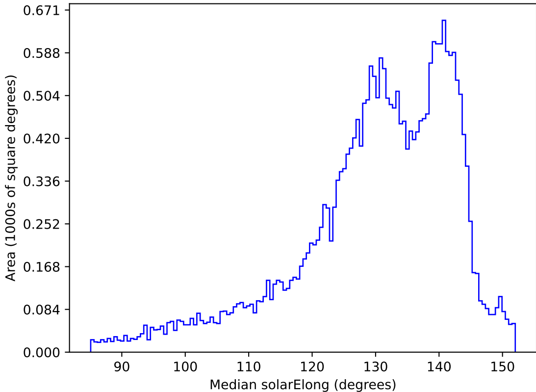
ddf_acor_sf10_lsf40_lsr20_v3.4_10yrs All sky all bands: Median solarElong
