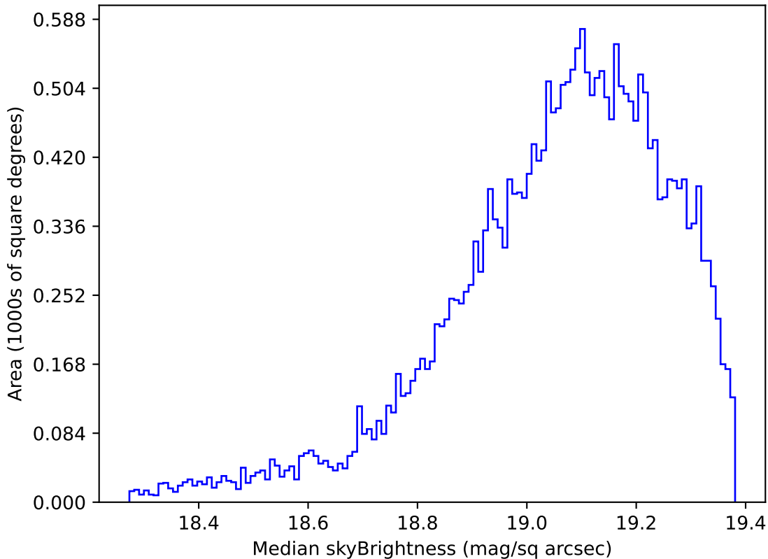
ddf_acor_sf10_lsf40_lsr20_v3.4_10yrs Yr 1 z band: Median skyBrightness
