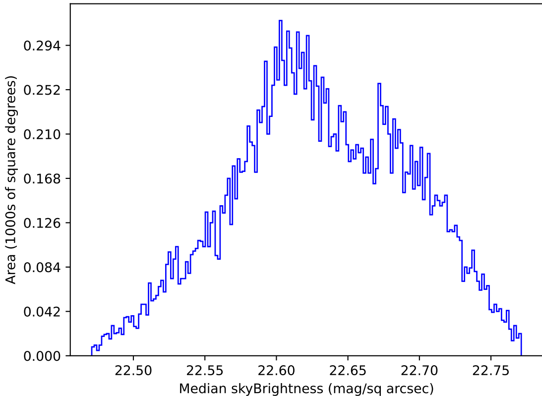
ddf_acor_sf10_lsf40_lsr20_v3.4_10yrs Yr 1 u band: Median skyBrightness
