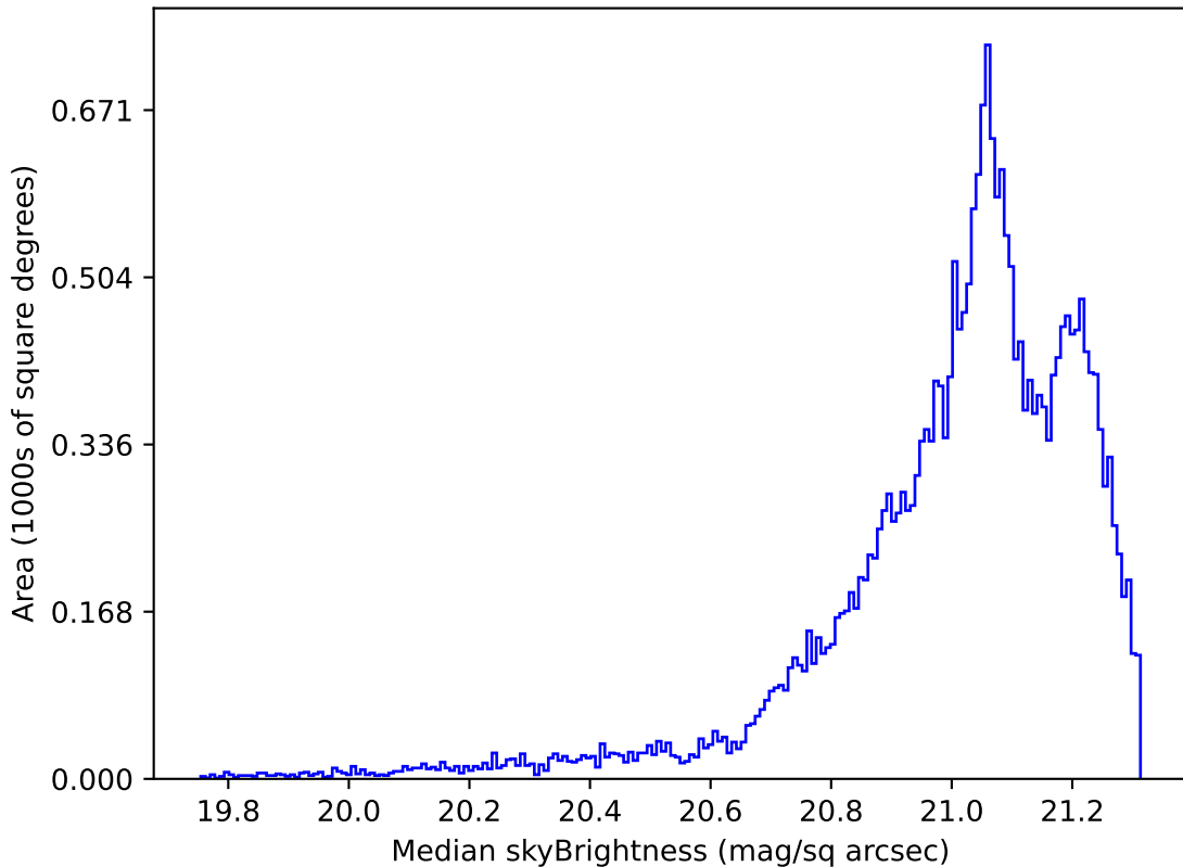
ddf_acor_sf10_lsf40_lsr20_v3.4_10yrs Yr 1 r band: Median skyBrightness
