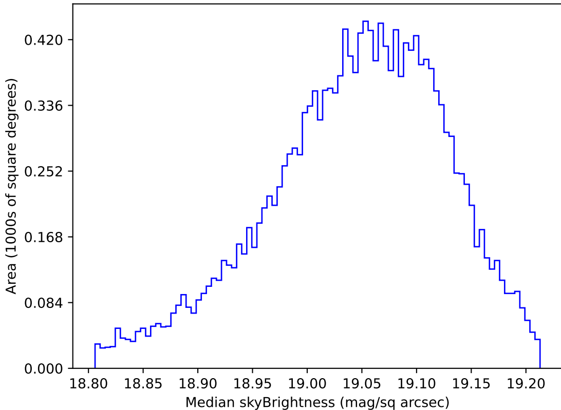
ddf_acor_sf10_lsf40_lsr20_v3.4_10yrs WFD z band: Median skyBrightness
