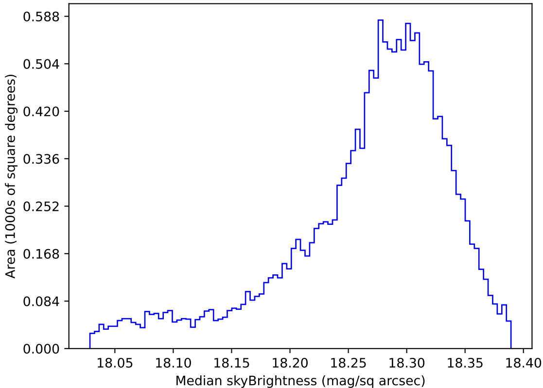
ddf_acor_sf10_lsf40_lsr20_v3.4_10yrs WFD y band: Median skyBrightness
