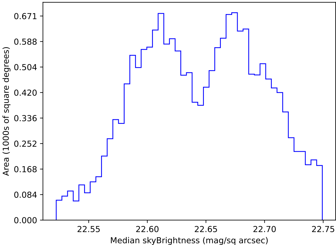
ddf_acor_sf10_lsf40_lsr20_v3.4_10yrs WFD u band: Median skyBrightness
