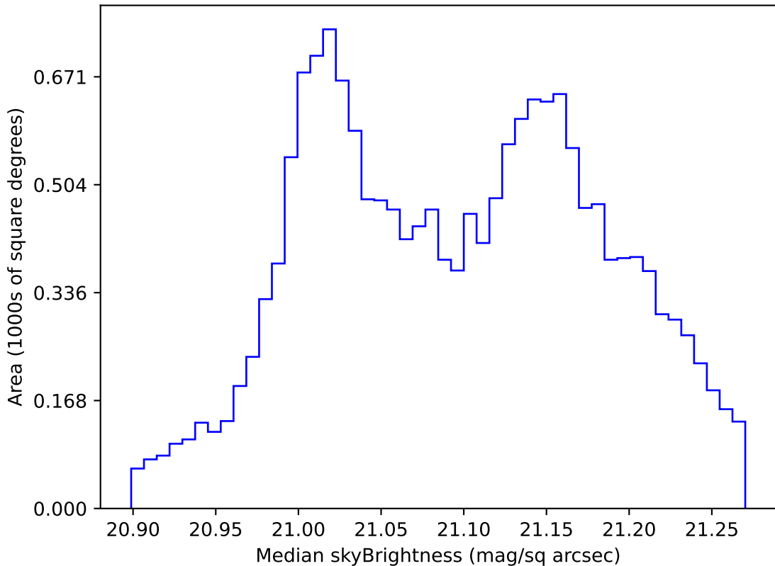
ddf_acor_sf10_lsf40_lsr20_v3.4_10yrs WFD r band: Median skyBrightness
