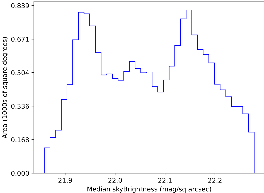
ddf_acor_sf10_lsf40_lsr20_v3.4_10yrs WFD g band: Median skyBrightness
