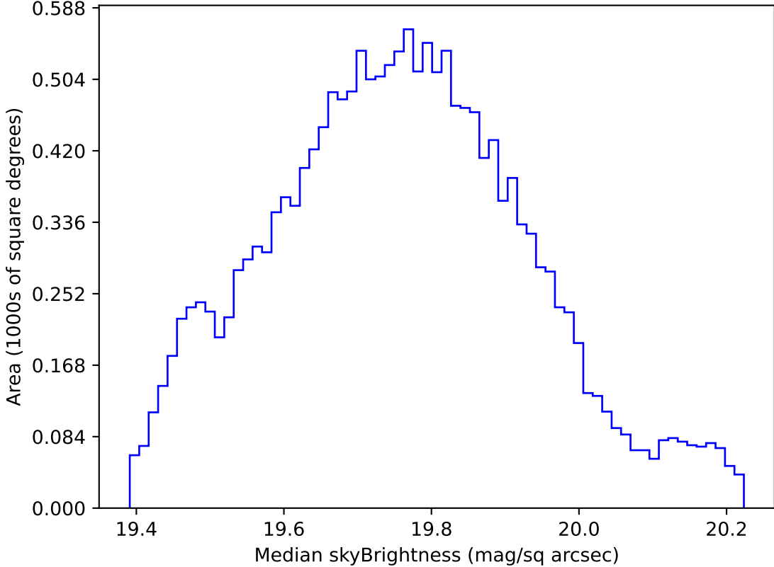
ddf_acor_sf10_lsf40_lsr20_v3.4_10yrs WFD all bands: Median skyBrightness
