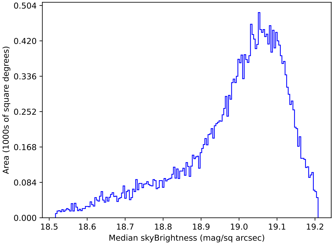
ddf_acor_sf10_lsf40_lsr20_v3.4_10yrs All sky z band: Median skyBrightness
