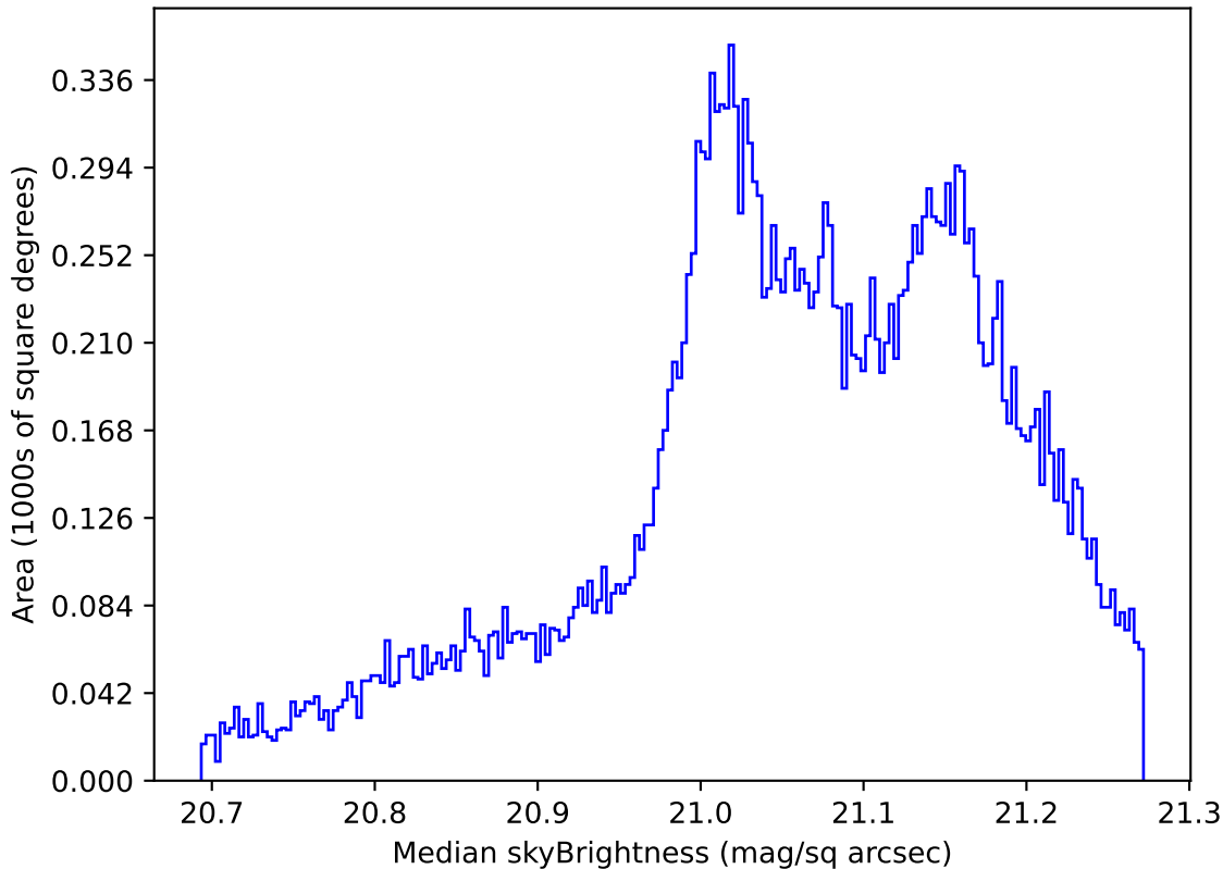
ddf_acor_sf10_lsf40_lsr20_v3.4_10yrs All sky r band: Median skyBrightness
