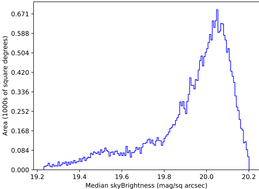
ddf_acor_sf10_lsf40_lsr20_v3.4_10yrs All sky i band: Median skyBrightness
