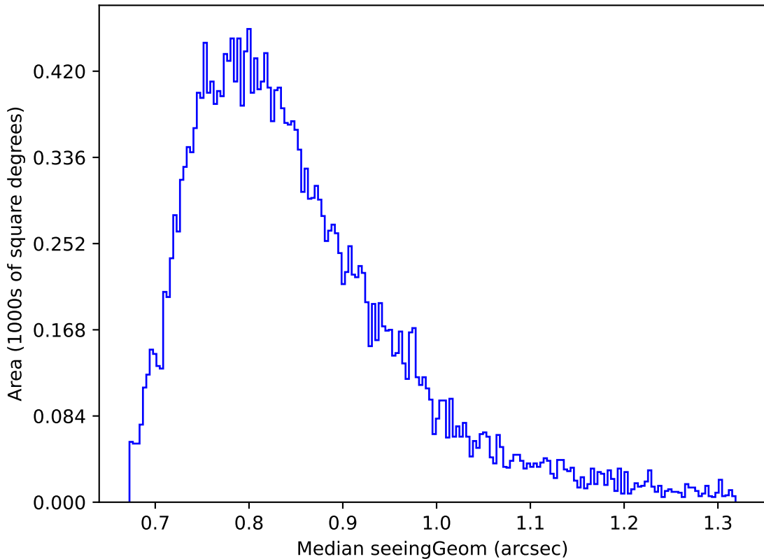
ddf_acor_sf10_lsf40_lsr20_v3.4_10yrs Yr 1 z band: Median seeingGeom
