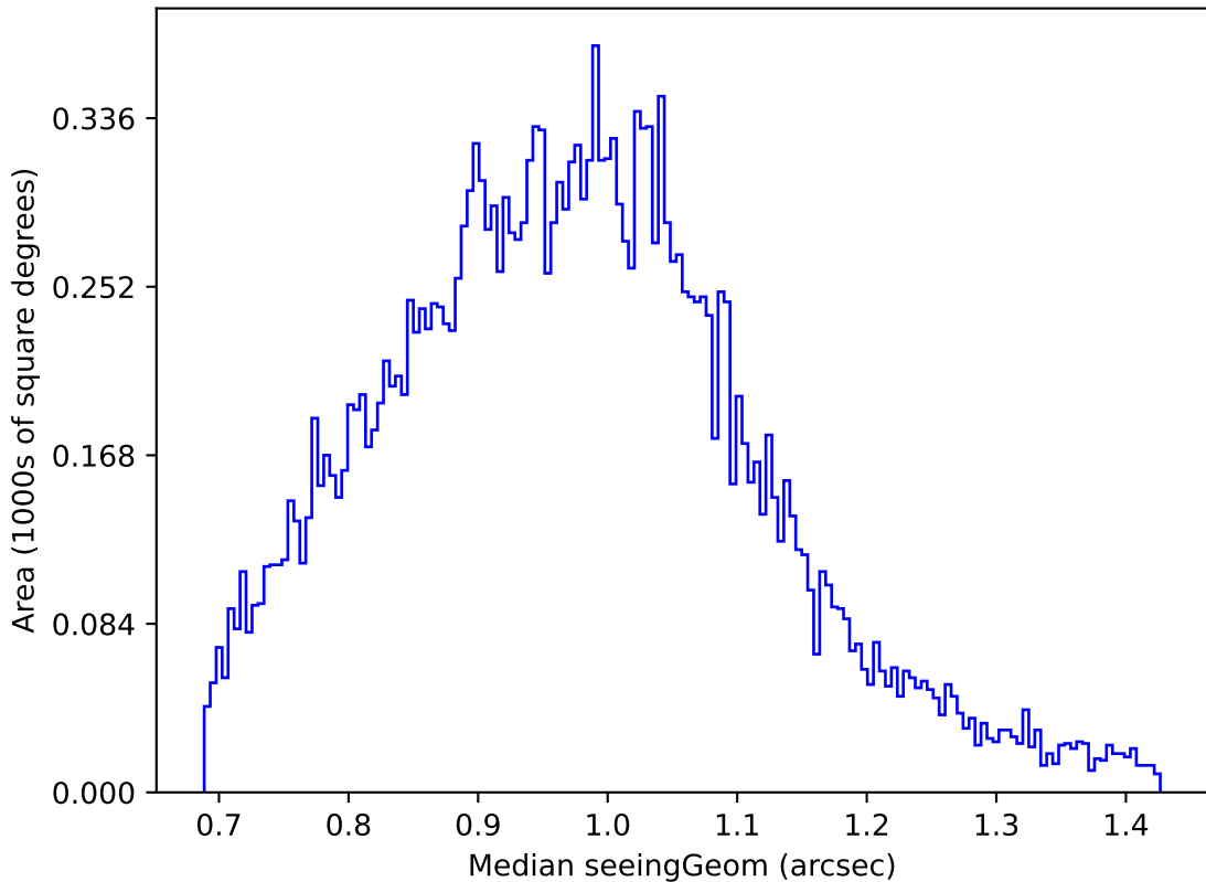
ddf_acor_sf10_lsf40_lsr20_v3.4_10yrs Yr 1 u band: Median seeingGeom
