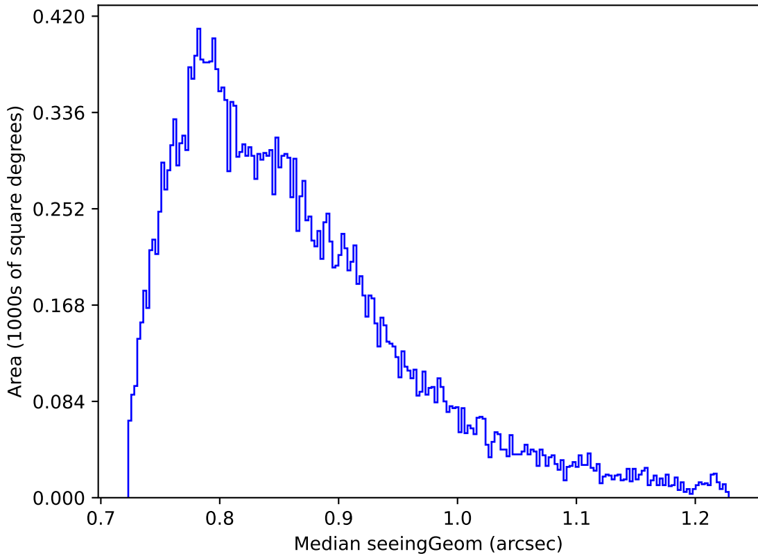
ddf_acor_sf10_lsf40_lsr20_v3.4_10yrs Yr 1 all bands: Median seeingGeom
