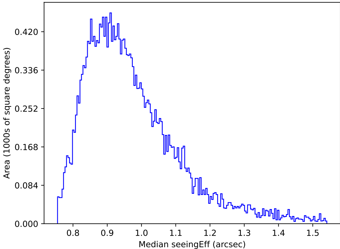
ddf_acor_sf10_lsf40_lsr20_v3.4_10yrs Yr 1 z band: Median seeingEff
