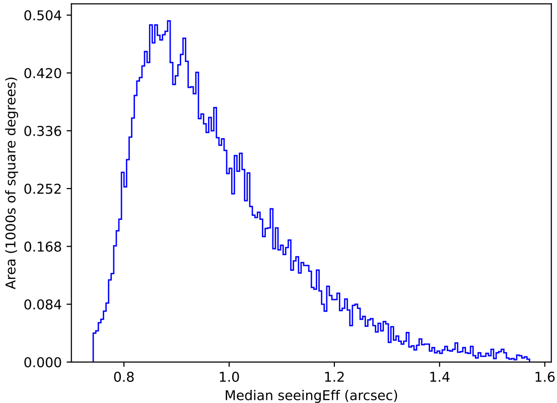
ddf_acor_sf10_ls40_lsr20_v3.4_10yrs Yr 1 r band: Median seeingEff
