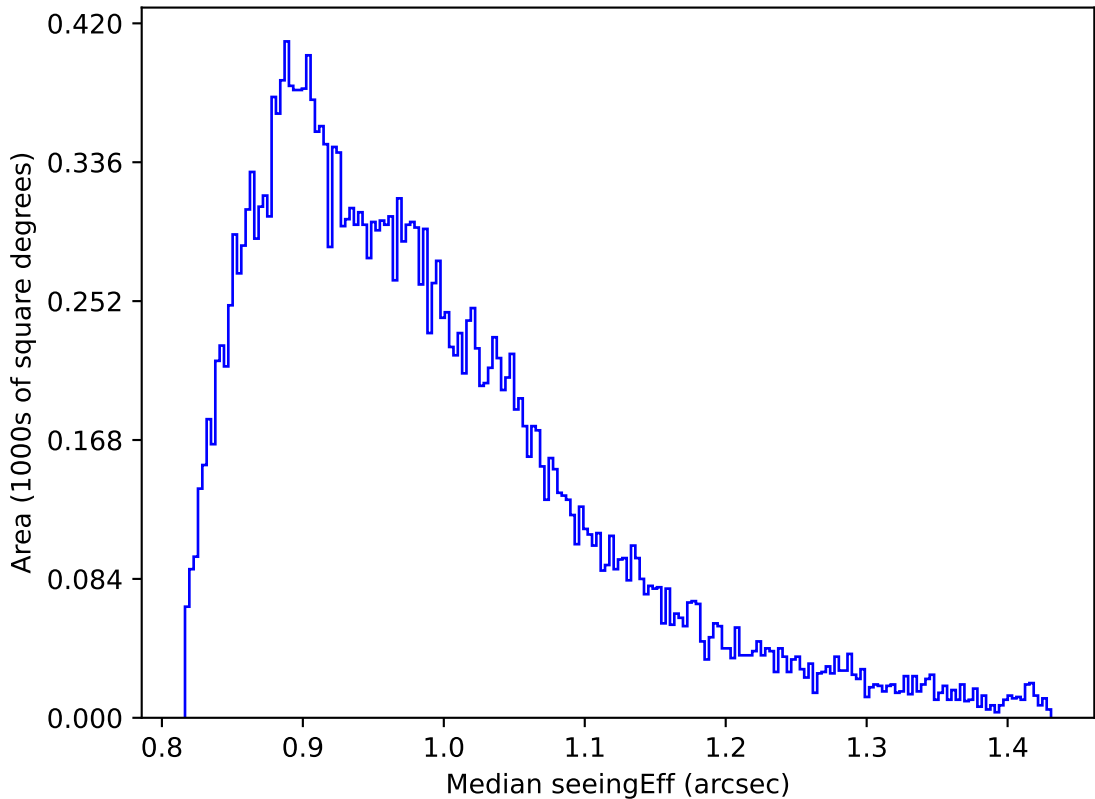
ddf_acor_sf10_lsf40_lsr20_v3.4_10yrs Yr 1 all bands: Median seeingEff
