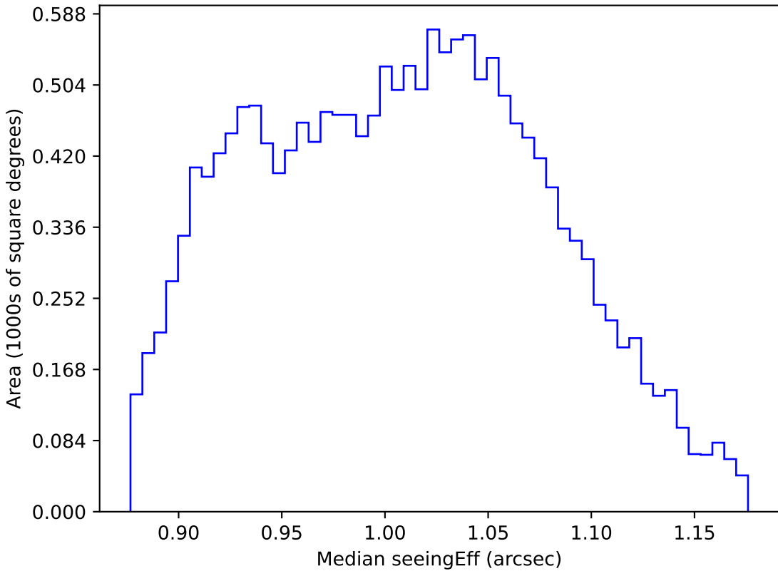
ddf_acor_sf10_lsf40_lsr20_v3.4_10yrs WFD z band: Median seeingEff
