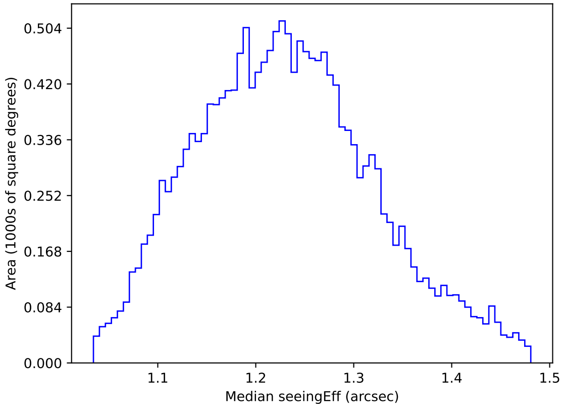
ddf_acor_sf10_lsf40_lsr20_v3.4_10yrs WFD u band: Median seeingEff
