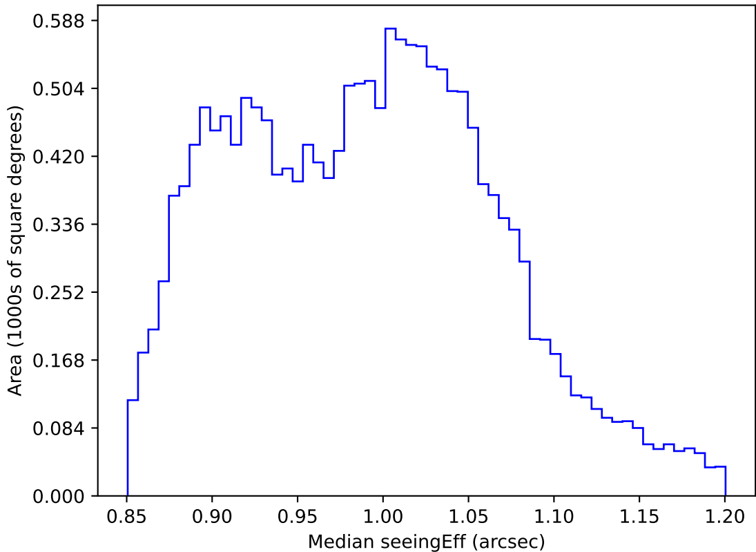
ddf_acor_sf10_lsf40_lsr20_v3.4_10yrs WFD i band: Median seeingEff
