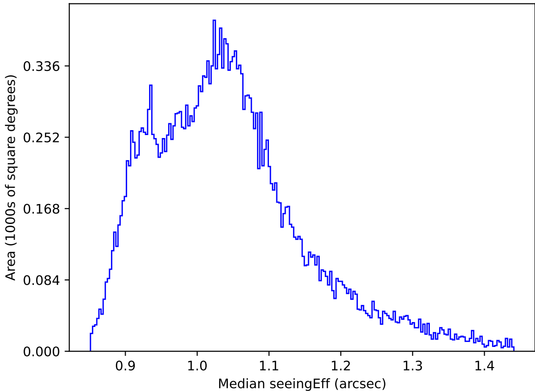
ddf_acor_sf10_lsf40_lsr20_v3.4_10yrs All sky z band: Median seeingEff
