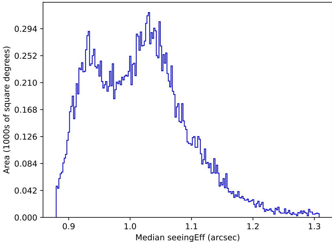
ddf_acor_sf10_lsf40_lsr20_v3.4_10yrs All sky y band: Median seeingEff
