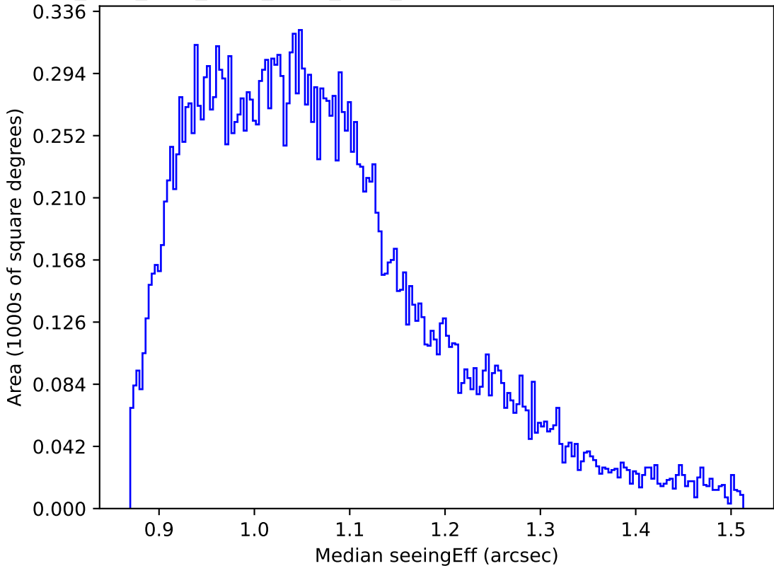
ddf_acor_sf10_lsf40_lsr20_v3.4_10yrs All sky r band: Median seeingEff
