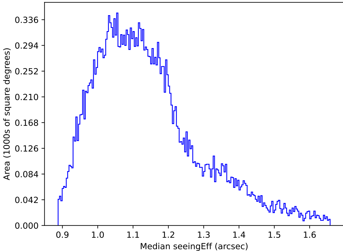
ddf_acor_sf10_ls40_lsr20_v3.4_10yrs All sky g band: Median seeingEff
