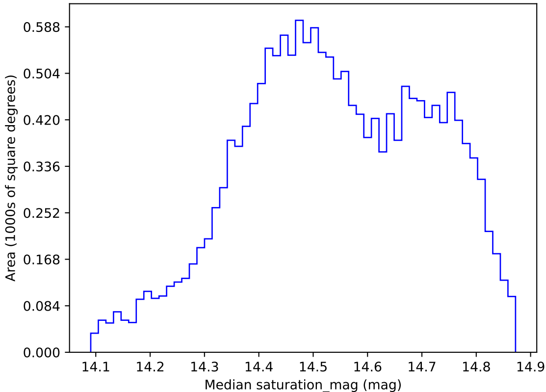
ddf_acor_sf10_lsf40_lsr20_v3.4_10yrs WFD i band: Median saturation_mag
