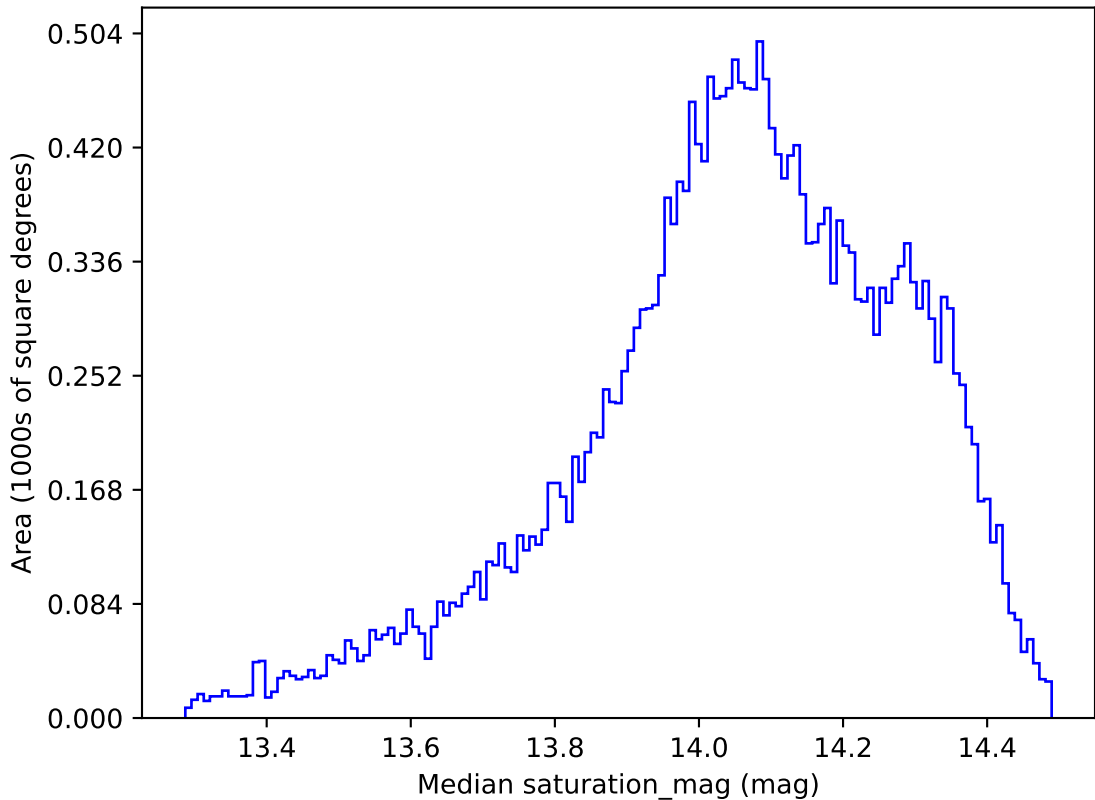
ddf_acor_sf10_lsf40_lsr20_v3.4_10yrs All sky z band: Median saturation_mag
