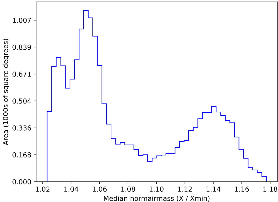
ddf_acor_sf10_lsf40_lsr20_v3.4_10yrs WFD all bands: Median normairmass
