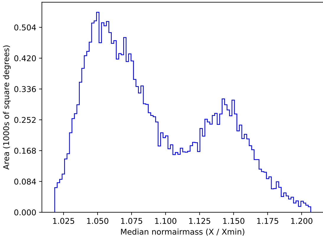
ddf_acor_sf10_lsf40_lsr20_v3.4_10yrs All sky y band: Median normairmass
