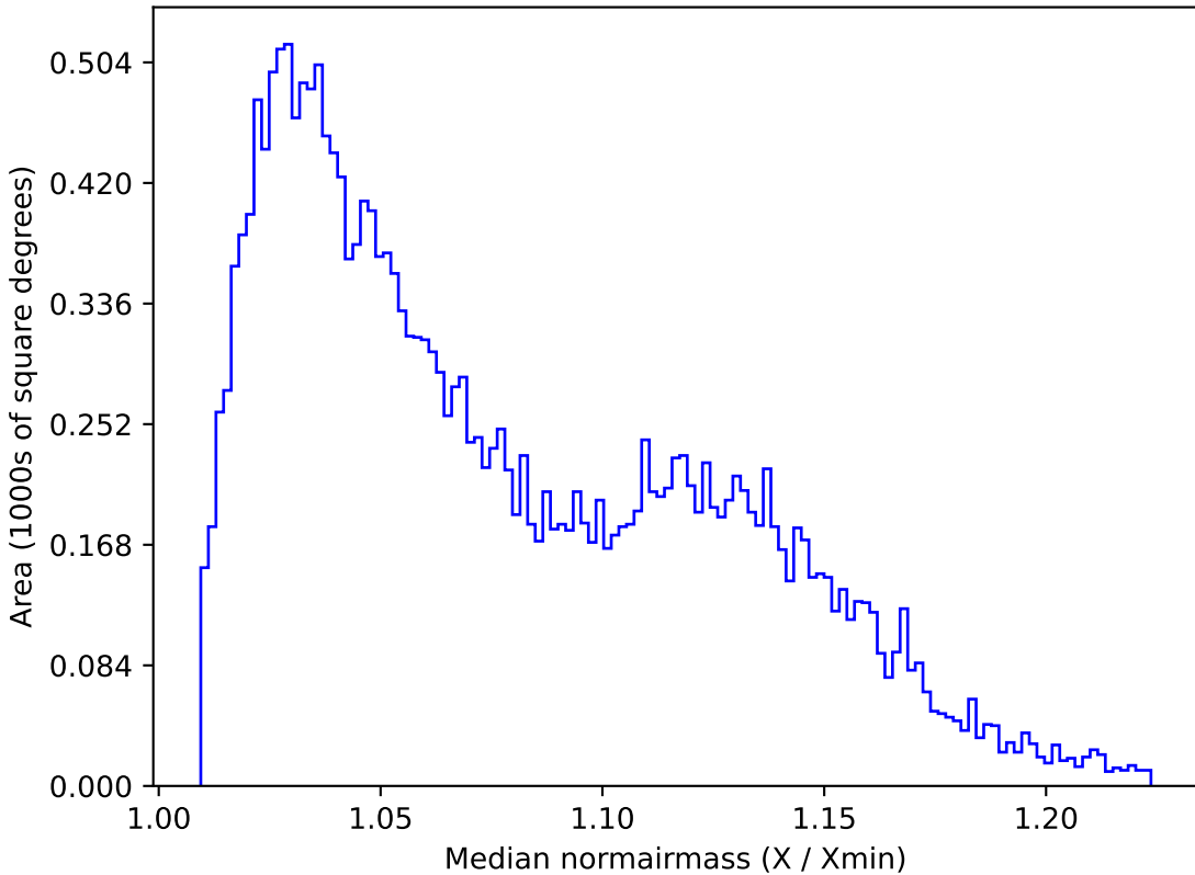
ddf_acor_sf10_lsf40_lsr20_v3.4_10yrs All sky u band: Median normairmass
