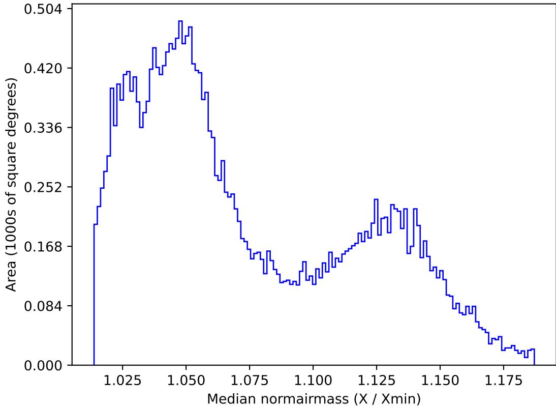
ddf_acor_sf10_lsf40_lsr20_v3.4_10yrs All sky r band: Median normairmass
