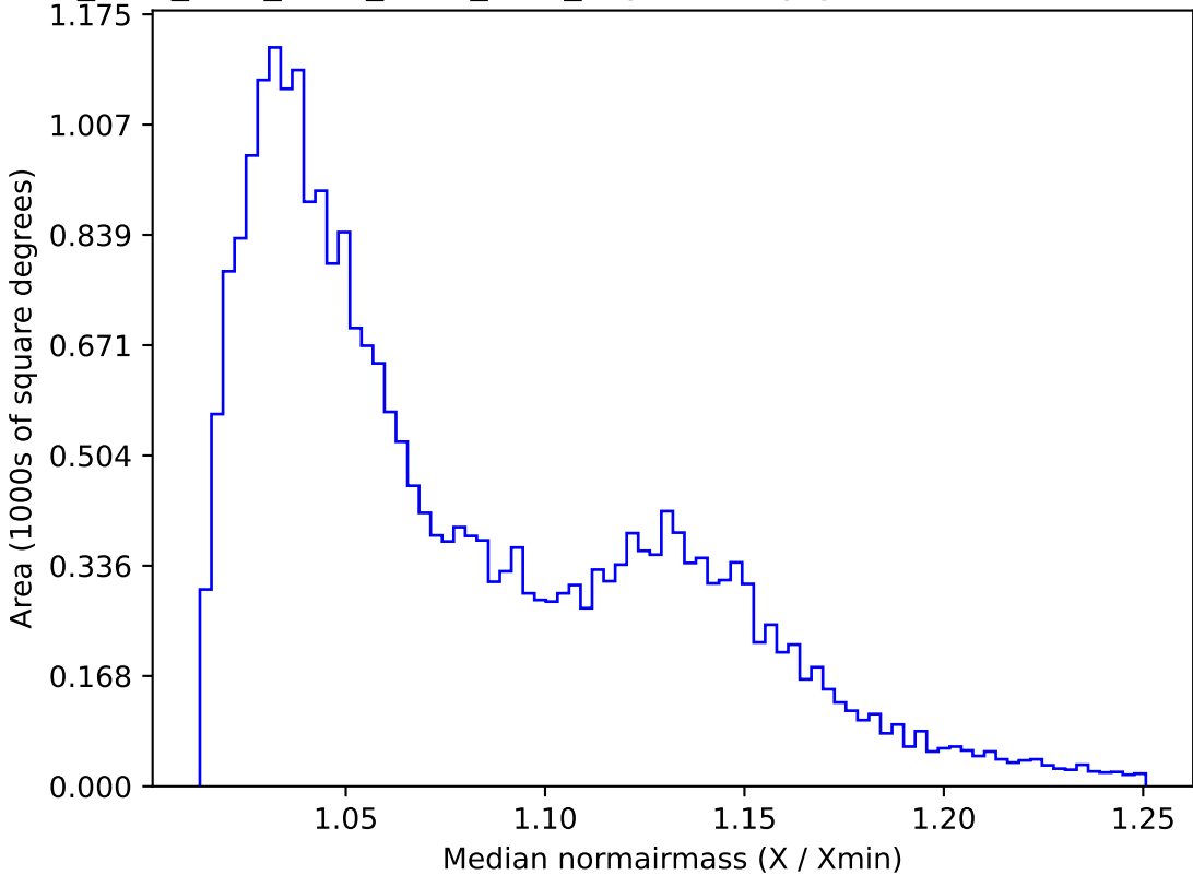
ddf_acor_sf10_lsf40_lsr20_v3.4_10yrs All sky g band: Median normairmass
