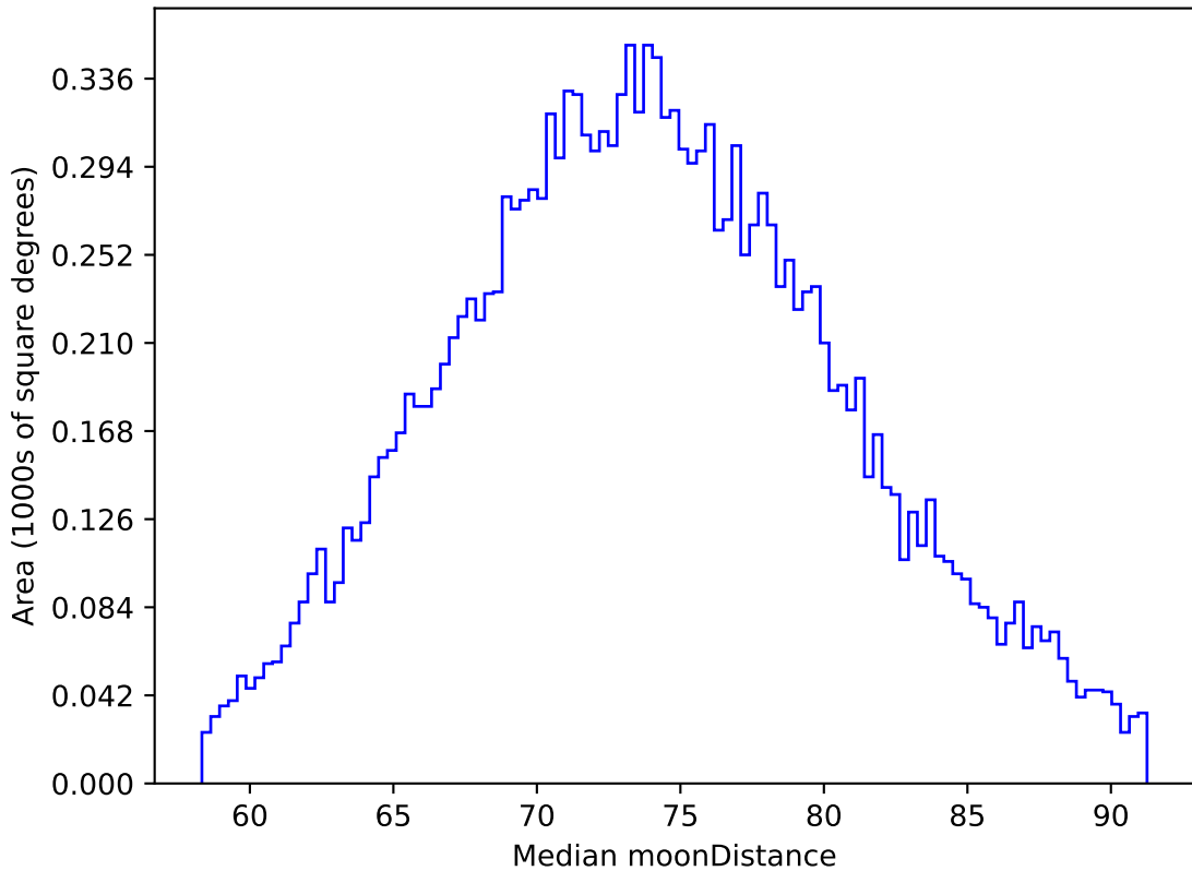
ddf_acor_sf10_lsf40_lsr20_v3.4_10yrs WFD z band: Median moonDistance
