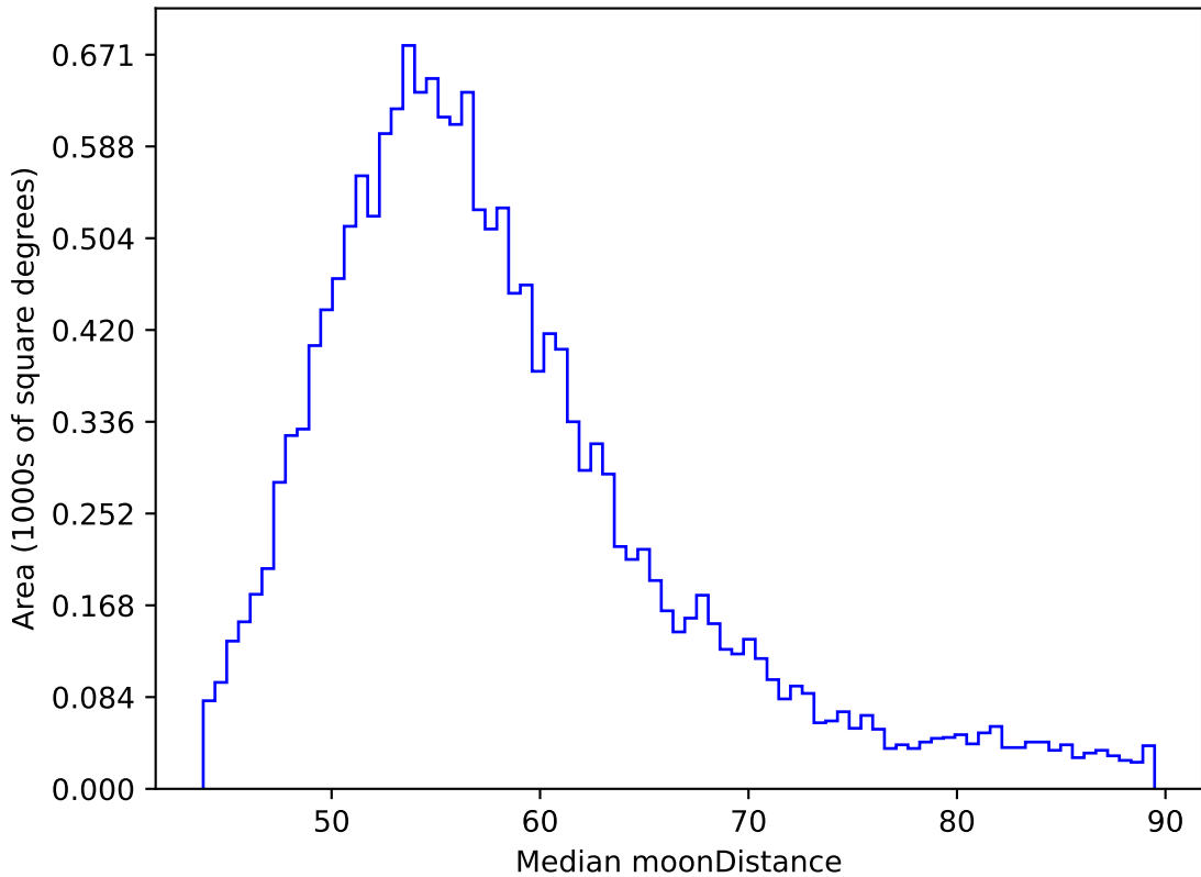
ddf_acor_sf10_lsf40_lsr20_v3.4_10yrs WFD y band: Median moonDistance
