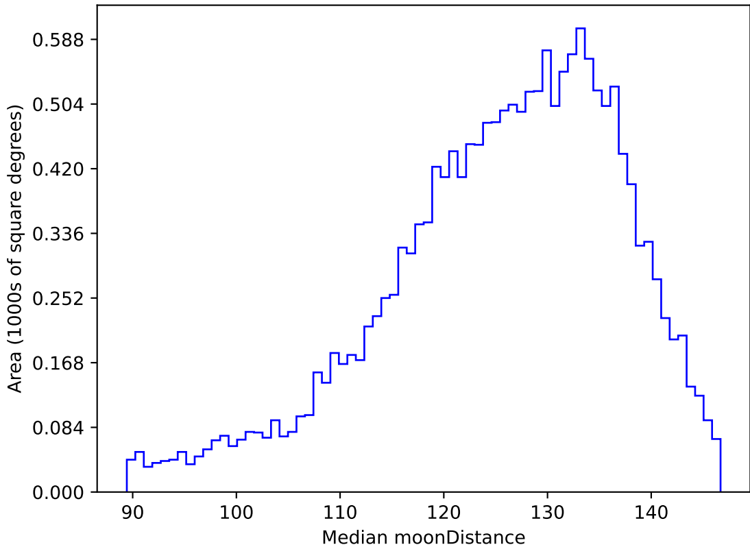
ddf_acor_sf10_ls40_lsr20_v3.4_10yrs WFD u band: Median moonDistance
