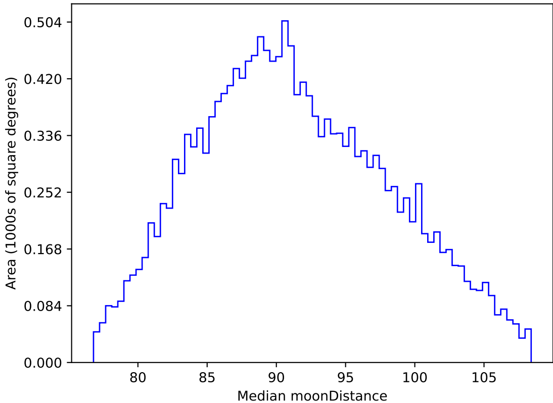
ddf_acor_sf10_lsf40_lsr20_v3.4_10yrs WFD i band: Median moonDistance
