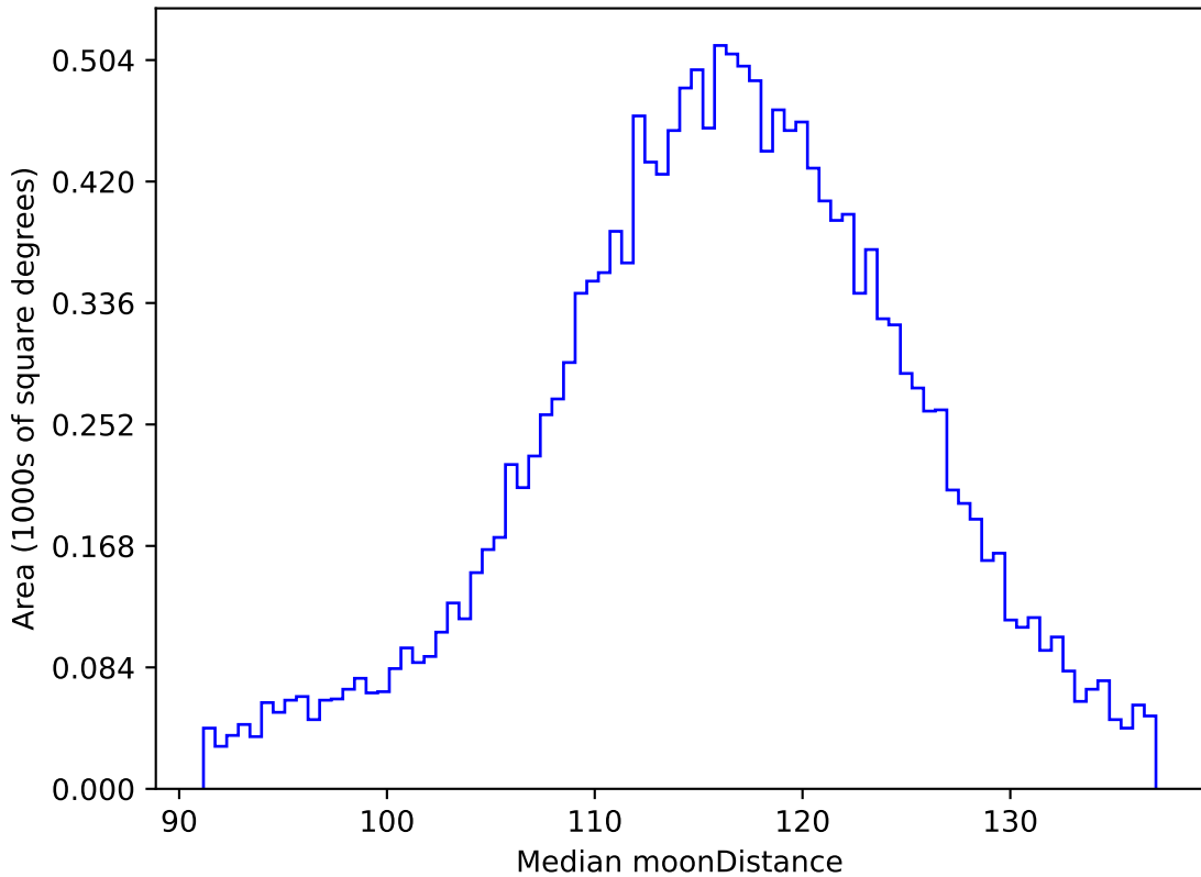
ddf_acor_sf10_lsf40_lsr20_v3.4_10yrs WFD g band: Median moonDistance
