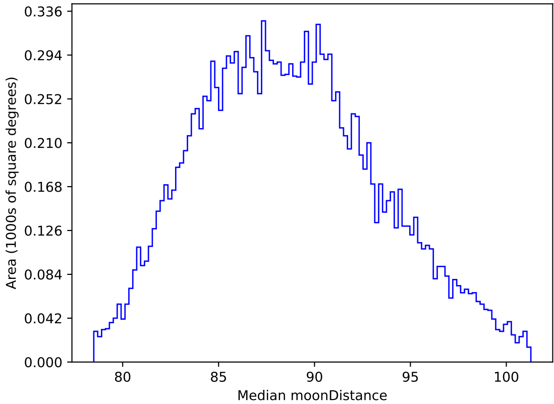
ddf_acor_sf10_lsf40_lsr20_v3.4_10yrs WFD all bands: Median moonDistance
