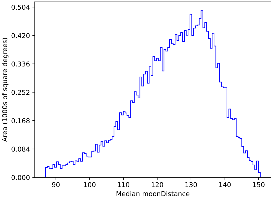
ddf_acor_sf10_lsf40_lsr20_v3.4_10yrs All sky u band: Median moonDistance
