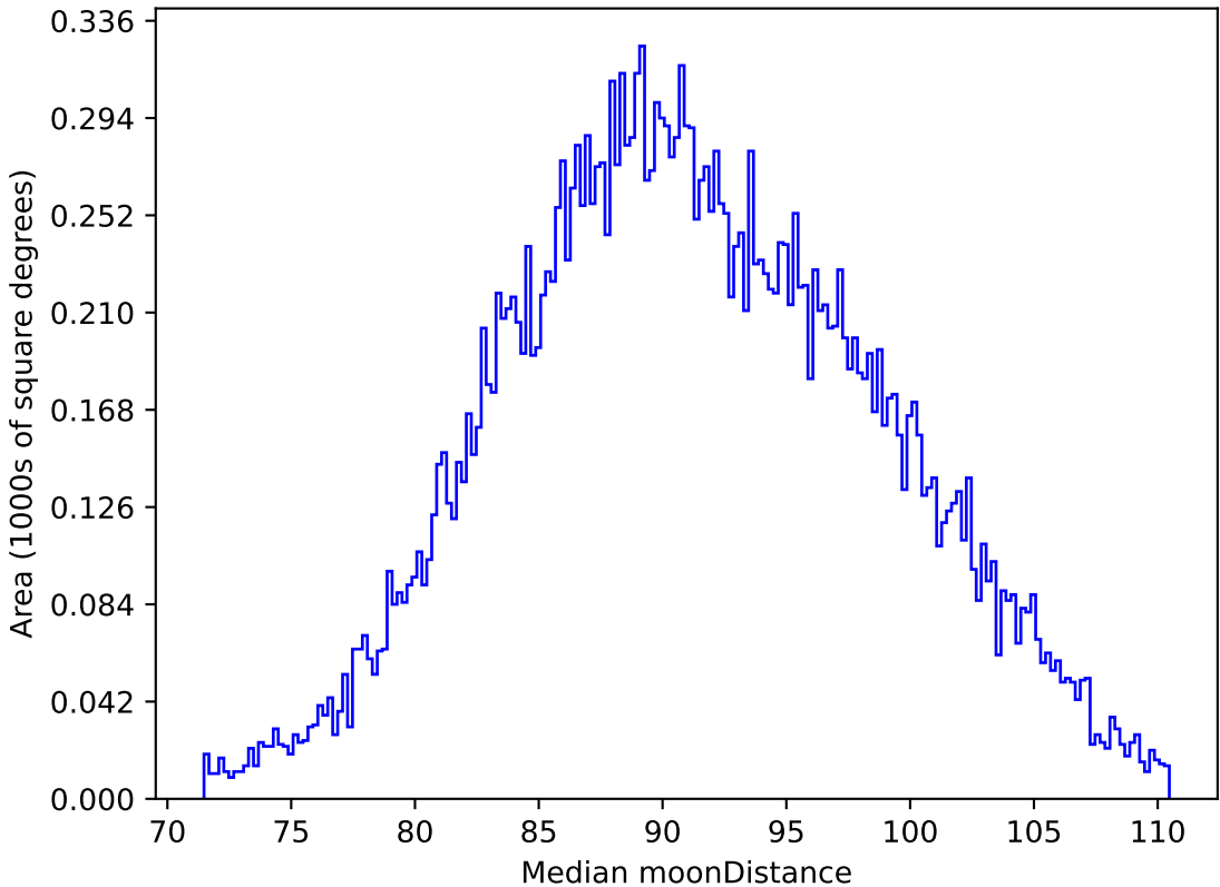
ddf_acor_sf10_lsf40_lsr20_v3.4_10yrs All sky i band: Median moonDistance
