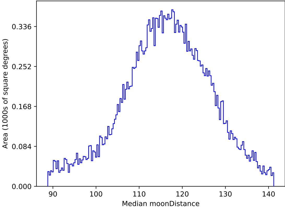
ddf_acor_sf10_lsf40_lsr20_v3.4_10yrs All sky g band: Median moonDistance
