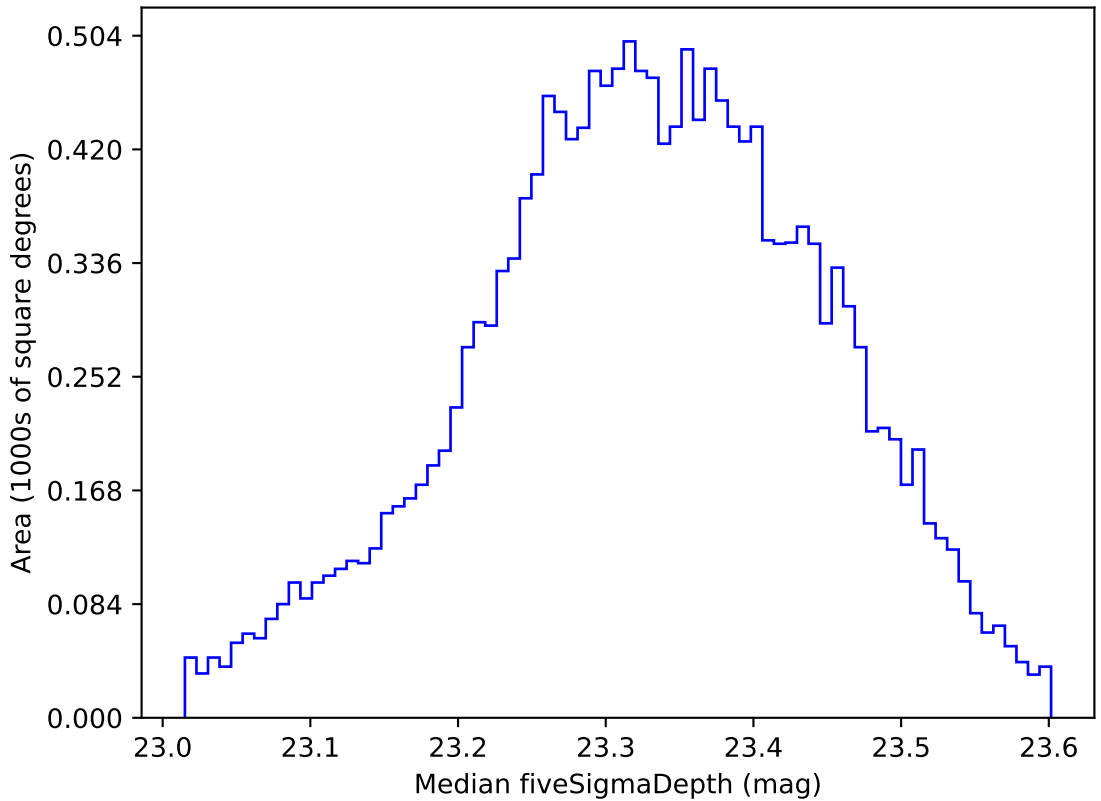
ddf_acor_sf10_lsf40_lsr20_v3.4_10yrs WFD all bands: Median fiveSigmaDepth
