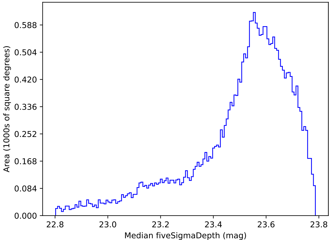
ddf_acor_sf10_lsf40_lsr20_v3.4_10yrs All sky i band: Median fiveSigmaDepth
