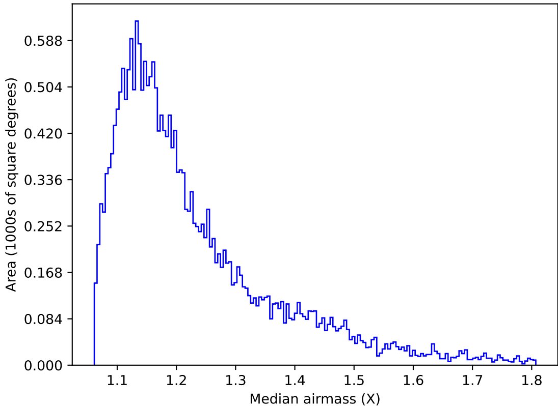
ddf_acor_sf10_lsf40_lsr20_v3.4_10yrs Yr 1 u band: Median airmass
